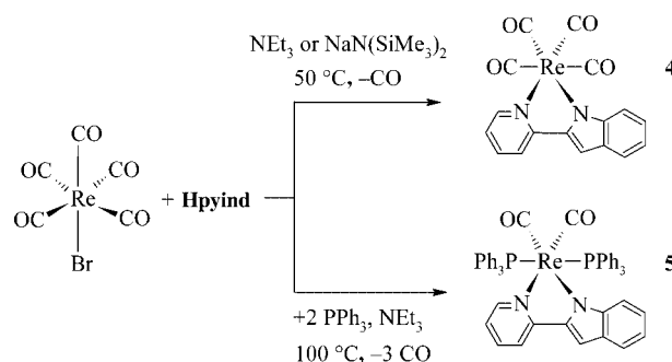
Scheme 4. Formation of complexes 4 and 5 .
