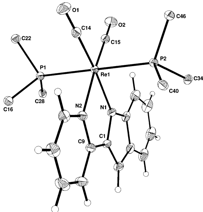
Figure 5. ORTEP plot of the rhenium compound 5 (25% probability). Only the terminal carbon atoms of both axial triphenylphosphane ligands are displayed. One disordered molecule of toluene is omitted.
