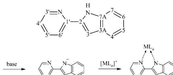
Scheme 1. General numbering (except crystal structures) and reaction scheme.
