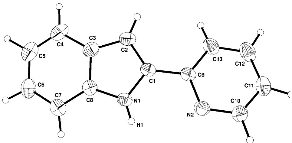
Figure 1. ORTEP plot (25% probability) of Hpyind. The numbering displayed is used in the discussion of all crystal structures for the pyind moiety.
