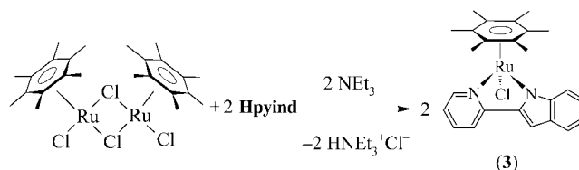
Scheme 3. Synthesis of ruthenium complex 3 .
