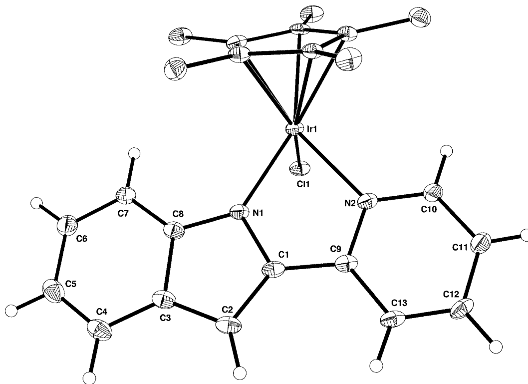
Figure 3. Molecular structure of complex 2 (25% probability). The methyl protons of C_5Me_5 are omitted.
