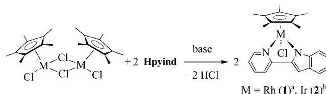
Scheme 2. Formation of rhodium and iridium complexes 1 and 2 ; a toluene, NaN(SiMe 3 ) 2 , 60 °C; b CH 2 Cl 2 , NEt 3 , 25 °C.
