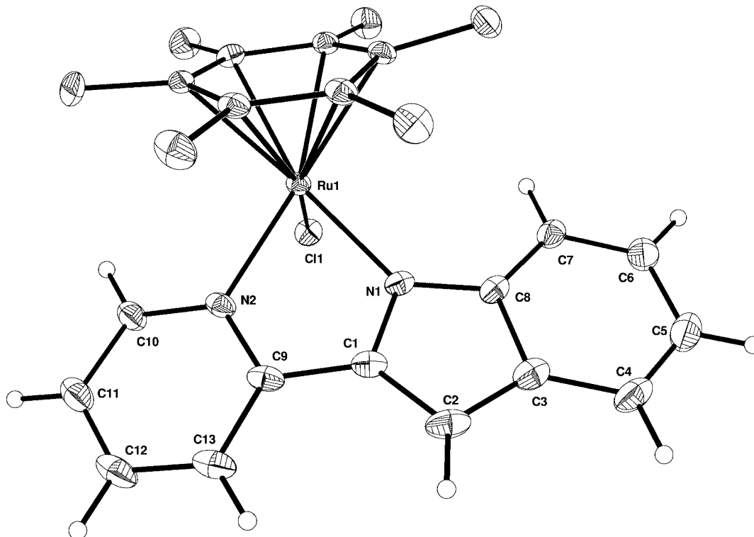
Figure 4. ORTEP plot of complex 3 (25% probability). The 18 disordered protons of the hexamethylbenzene moiety are omitted and a solvent molecule of CH_2Cl_2 is not included in the diagram.
