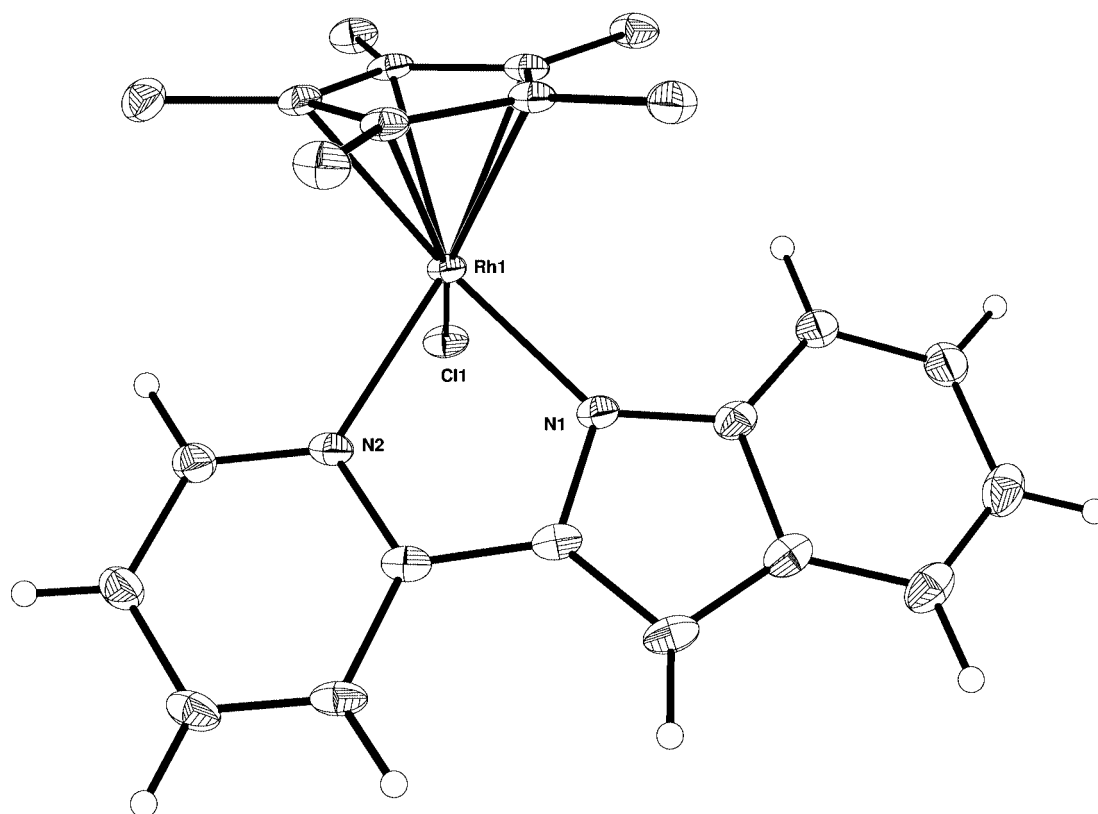
Figure 2. Molecular structure of rhodium complex 1 (25% probability). The methyl protons of C 5 Me 5 are omitted for clarity.
